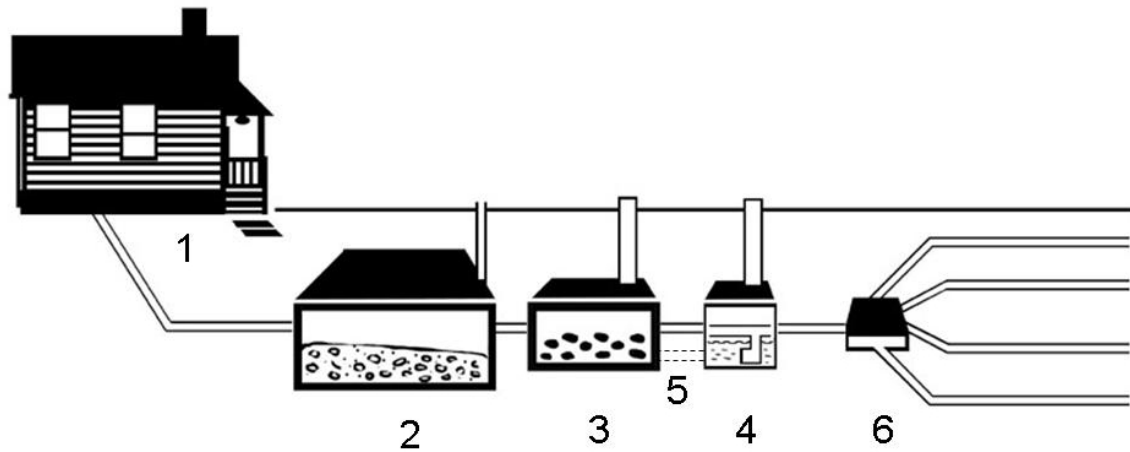
Figure 1. Recommended system design for on-site wastewater disposal systems for installation on existing mines (conceptual, not to scale). Legend:
